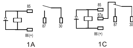
1A 1C Wiring diagram (Bottom view)
