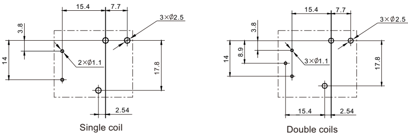
Mounting (Bottom view)
