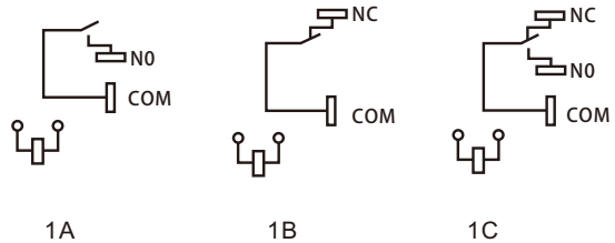
Wiring diagram
