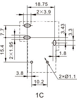
Mounting (Bottom view)
