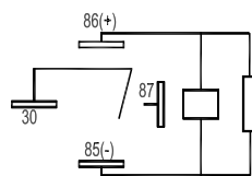
With resistor
