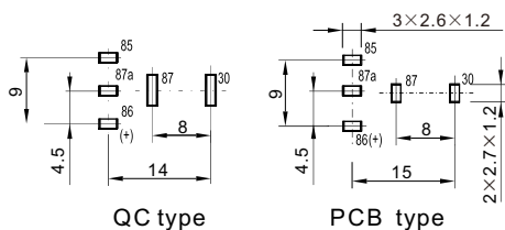
Mounting (Bottom view)
