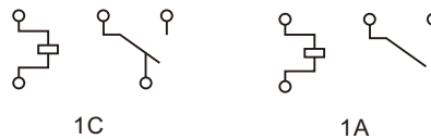
Wiring diagram (Bottom view)
