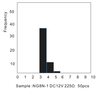
NC Contact Resistance (mΩ)
